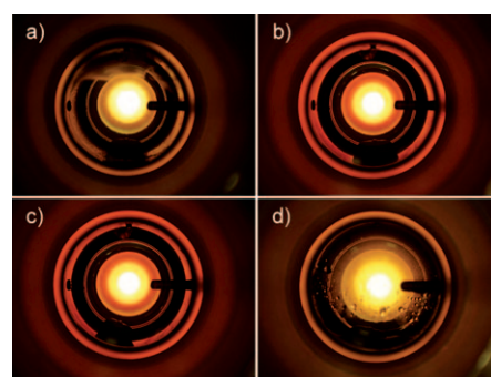
Figure 3. Photographs showing the phase behavior at 55 °C of a mixture containing 3 (5.23 mmol) and DMC (0.0113 mmol) with a mixture of scCO 2 (0.432 mol) and N 2 (10.5 mmol) using a variable volume view cell [35] a) 120 bar: multiphase mixture, b) 140 bar: single phase, c) 180 bar: also single phase, d) separate experiment with the product mixture (replacing 3 with the 100% converted mixture of peroxide products in the same molar ratios). Note the droplets indicating a biphasic mixture with scCO 2 under all conditions studied (40–60 °C, 100–200 bar).
