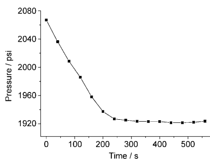
Figure 4. Monitoring the batch photo-oxidation of 3 (0.328 mmol) and DMC (0.709 mmol) with O 2 (0.595 mmol) in scCO 2 (2067 psi) at 40 °C. The batch cell was irradiated using a single white 1000 lumen LED. The pressure drop corresponds to one molar equivalent of O 2 being consumed for each mole of 3 present.
